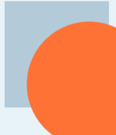
source-over
